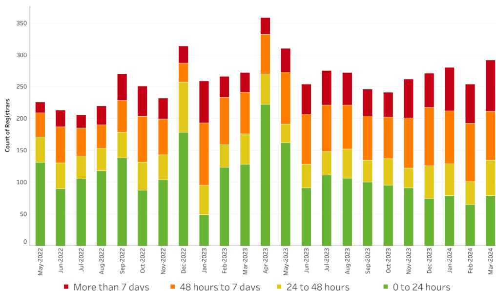
Figure 6: Registrar Median Mitigation Time
