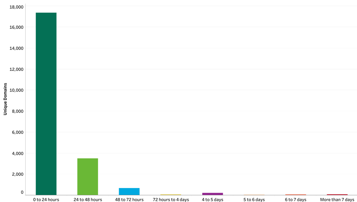
Figure 7: Median Mitigation Time 2025-06
