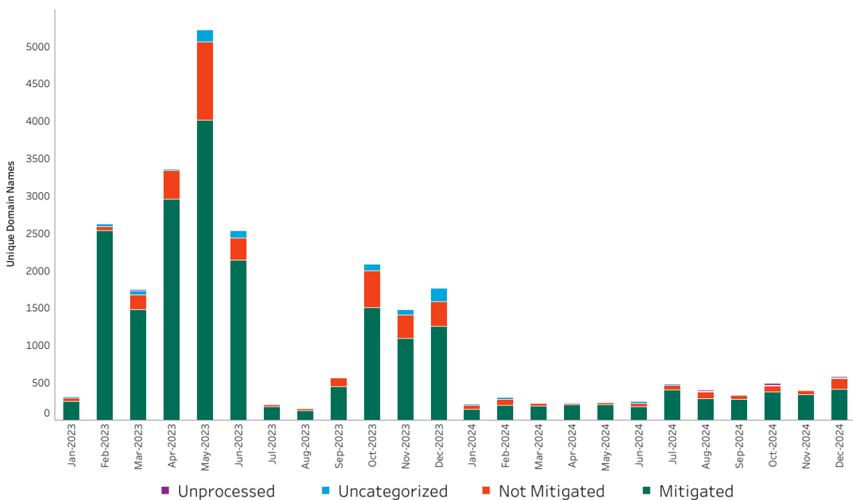
Figure 5: Mitigation - Malware
