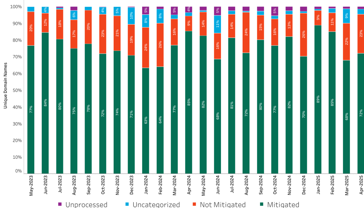
Figure 5: Mitigation - Malware
