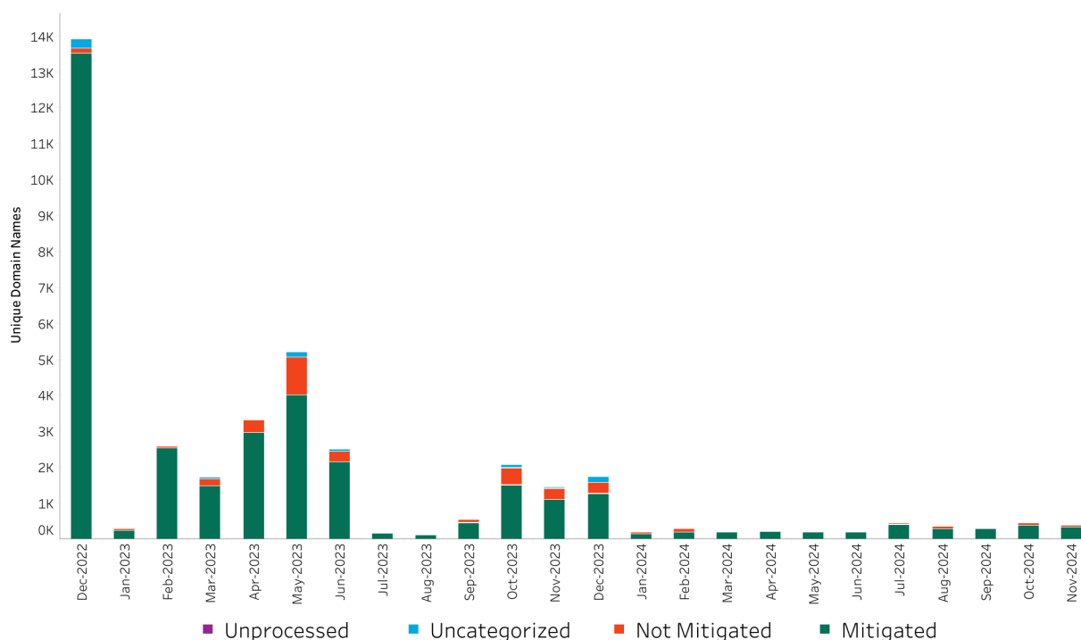
Figure 5: Mitigation - Malware
