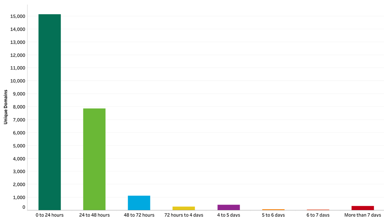
Figure 7: Median Mitigation Time 2025-07
