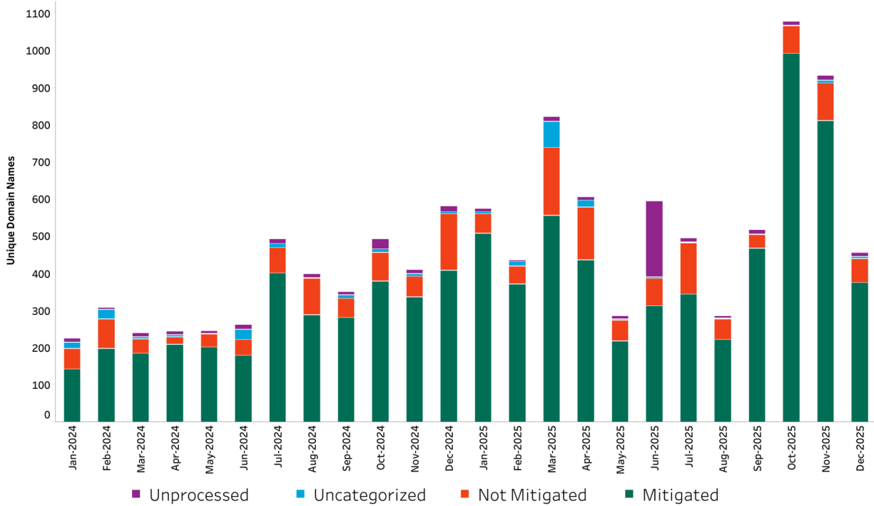
Figure 5: Mitigation - Malware
