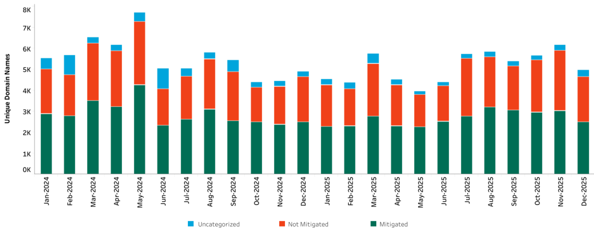
Figure 5.1: Mitigation - Compromised
